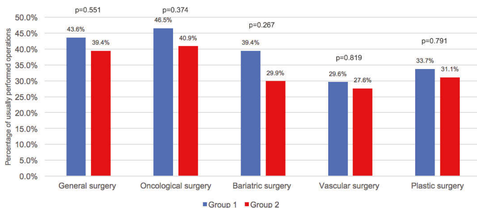
Fig. 2. Mean percentage of the norm performed during pandemic, for various types of surgery (Group 1 — COVID-19-dedicated hospitals; Group 2 — non-COVID-19-dedicated hospitals; Student’s t-test was used to compare Group 1 and 2).
